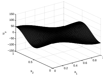
FIG. 6.19. Control u_\mu
