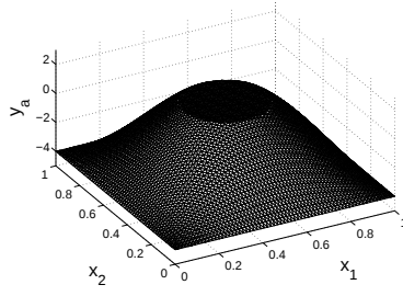
FIG. 6.32. State constraints y_c
