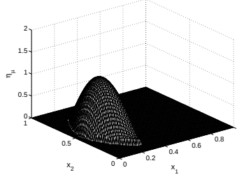
FIG. 6.22. Multiplier \eta_\mu
