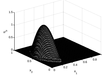
FIG. 6.30. Control \eta_\mu at \mu = 10^{-6}
